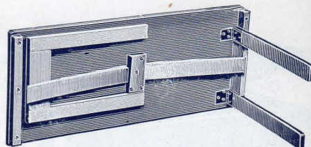
No. 380. —Showing method of folding.
