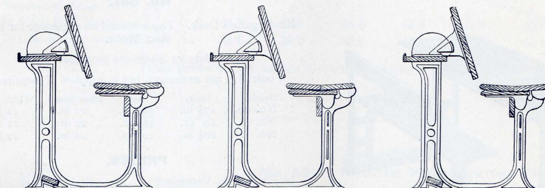
Section showing Desks arranged as Seats, facing opposite direction to that shown in previous section.
