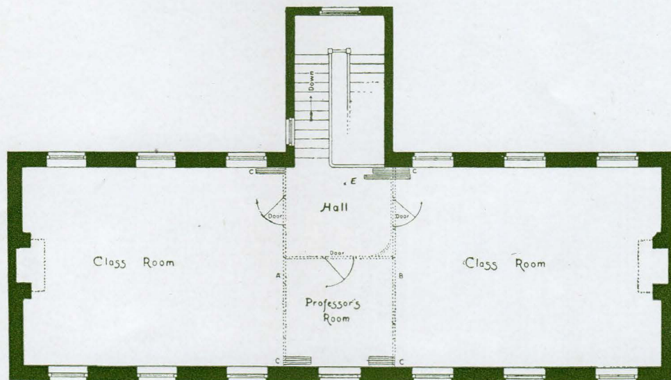
PLAN. Showing an Unusual Arrangement of Sub-Division and Folding.
