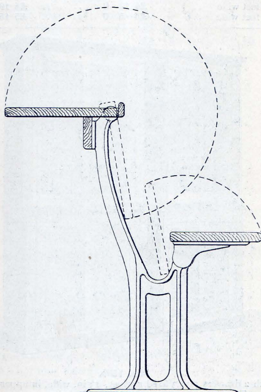
Section of No. 525.
