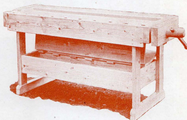
No. 921—Manual Bench.
