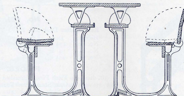
Section showing two Desks arranged as a Table, the seats being used either with or without a back support.
