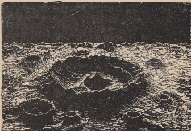
Volcanes lunares.
